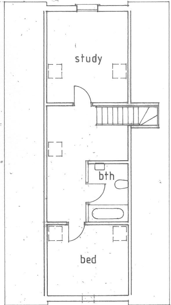
FIRST 1:100
